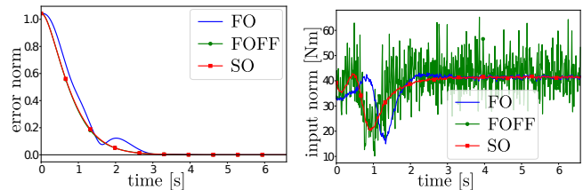
Fig. 3. Comparison of visual error (left) and control inputs (right) when noise is injected in simulations. FOFF and SO are still almost indistinguishable in terms of error evolution.
