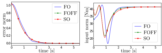
Fig. 2. Comparison of the visual error (left) and control input (right) using the different control strategies, in absence of noise. FOFF and SO are almost indistinguishable in terms of error evolution.
