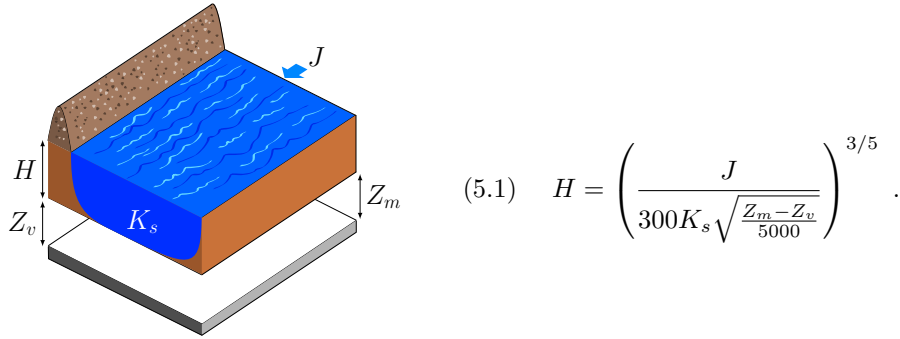
Fig. 1: Simplified river cross section.
