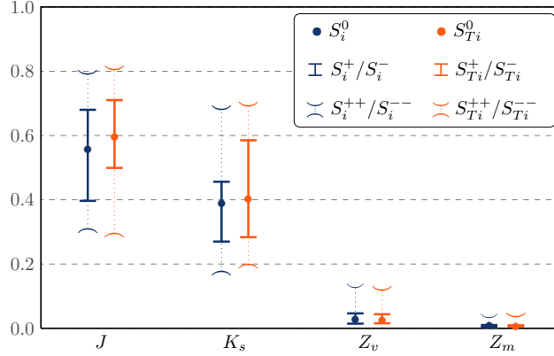
Fig. 3: Different definitions of robustness for the Sobol indices yield different bounds.
