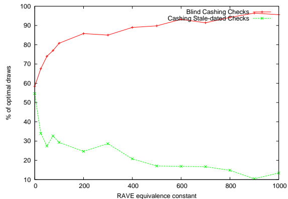
Figure 2: The percentage of matches with optimal moves of both players at Blind Cashing Checks and Cashing Stale-dated Checks as a function of the RAVE equivalence constant.
