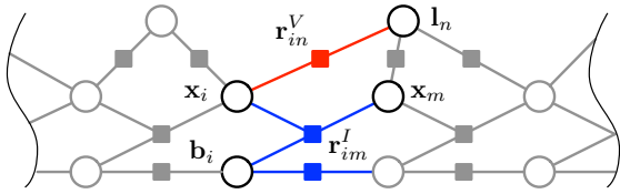
Fig. 1. A typical fraction of the factor graph, involving state blocks corresponding to keyframes \mathbf{x}_i = (\mathbf{p}_i, \mathbf{v}_i, \mathbf{R}_i) , biases \mathbf{b}_i and landmark poses \mathbf{l}_n . IMU factors (blue) relate consecutive keyframes and the IMU biases. The lower branch controls bias drift along time. Visual factors (red) relate landmarks with poses (\mathbf{p}_i, \mathbf{R}_i) .
