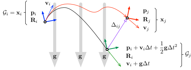
Fig. 2: The free-falling, non-rotating frame \mathcal{G}_t follows a parabolic trajectory governed only by gravity \mathbf{g} and determined by the initial conditions \mathbf{p}_i , \mathbf{v}_i and \mathbf{R}_i at time i ( \mathcal{G}_i = \mathbf{x}_i , blue). The IMU delta \Delta_{ij} between times i and j is defined as the state of the IMU at time j ( \mathbf{x}_j , red) expressed in the free-falling frame at time j ( \mathcal{G}_j , green).
