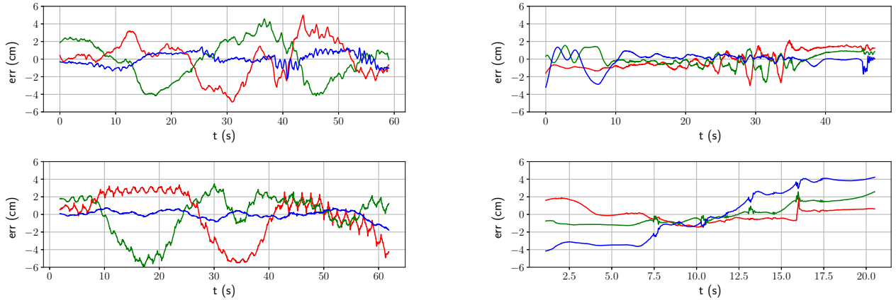
Fig. 6: Translation estimation error (cm) as a function of time (s). In the clock-wise sens, starting from the top-left corner, the datasets are handheld camera, stairs climbing, stairs descending and walking on flat ground. RGB colors correspond to xyz axes.
