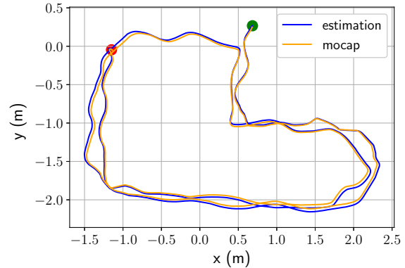
Fig. 5: Two loops of the experimental field with camera in hand
