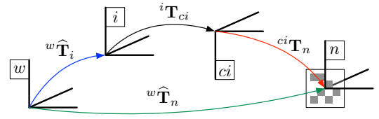
Fig. 4: Kinematic chain of the reference frames involved in one tag observation and their transforms \mathbf{T} \in SE(3) . w : world frame; i : IMU frame at time i ; ci : camera frame at time i ; n : tag n frame. The SE(3) tag measurement is highlighted in red.
