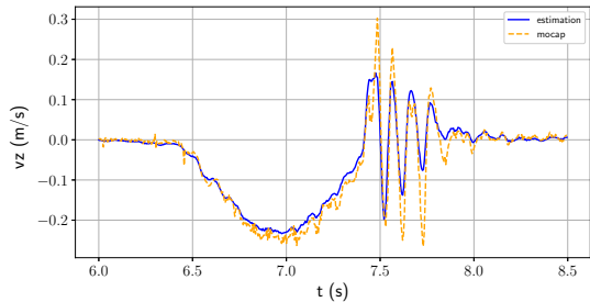
Fig. 7: Descending stairs (one step): the robot first lowers its center of mass and then touches the next step with results in vibrations from the impact.
