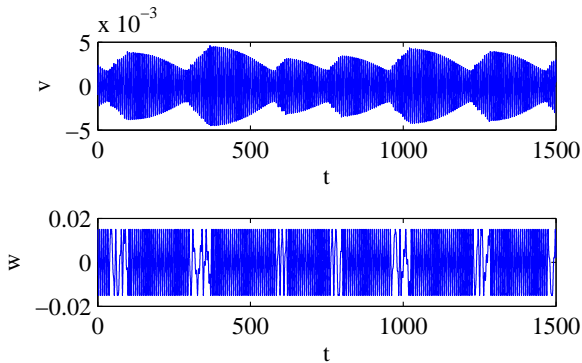
FIGURE 7. Numerical integration of Eqs. (4) and (5) for the set of parameters (25).
