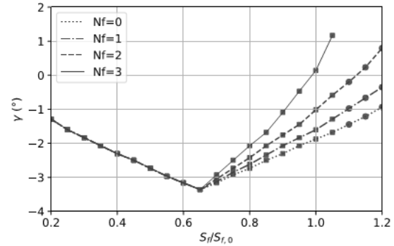
Figure 6 : Maximum descent angle in landing conditions as a function of vertical tail relative surface area and number of engine failure.
