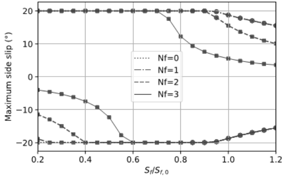
Figure 4: Maximum positive and negative \beta at V_2 in take-off conditions. N_f refers to number of failed engine. Rectangles show saturation of engines and circles show limit of bank angle.
