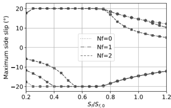
Figure 5: Maximum positive and negative \beta at 1.3V_{sr} in take-off conditions. N_f refers to number of inoperative engines. Rectangles show saturation of engines and circles show limit of bank angle
