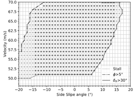
Figure 2: Twin engine ATR72 with one engine failure
