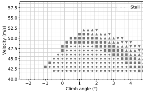
Figure 7: Flight envelop in landing condition with three inoperative engines and S_f/S_{f_0} = 1
