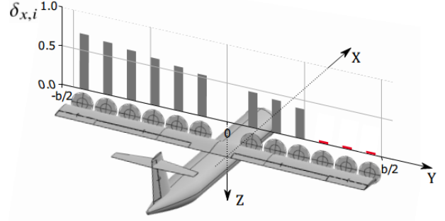
Figure 1 : Illustration of an ATR72 with distributed propulsion, differential thrust and engine failures.
