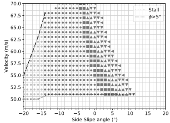
Figure 3: DEP ATR72 using differential thrust only and three engine failures as shown in Fig. 1.
