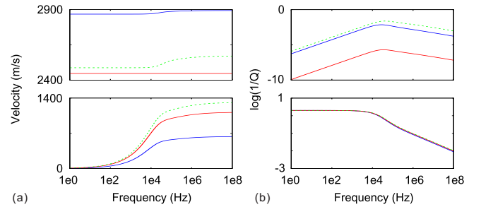
Figure 4: Variation of the phase velocity (a) and of the attenuation (b) with frequency for different values of porosity. The horizontal axis is shown with a logarithmic scale. The thick-solid blue, thin-solid red, and thin-dashed green lines present the results for \phi = 0.05 , 0.24 and 0.45 , respectively. The upper and lower panels present the results for P1 and P2 waves, respectively.
