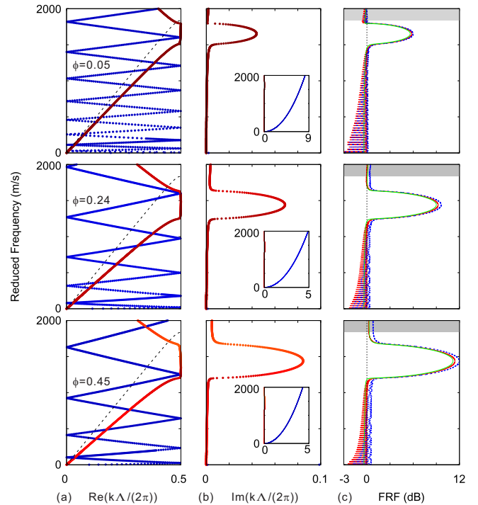
Figure 7: Influence of porosity on the complex band structures for 1D FSPMs. Panels (a) and (b) show the variation of the reduced frequency with the real and imaginary parts of the reduced wavenumber. The dashed lines are the dispersion curves for \phi = 0 . The colorscale is the same as that in Fig. 2. FRF curves for a finite metamaterial with 50 periods are shown in panel (c). The red solid and blue dashed lines represent the results for the excitation of u_x and w_x , respectively. The green lines present the results of Eq. (19) for the P1 wave.
