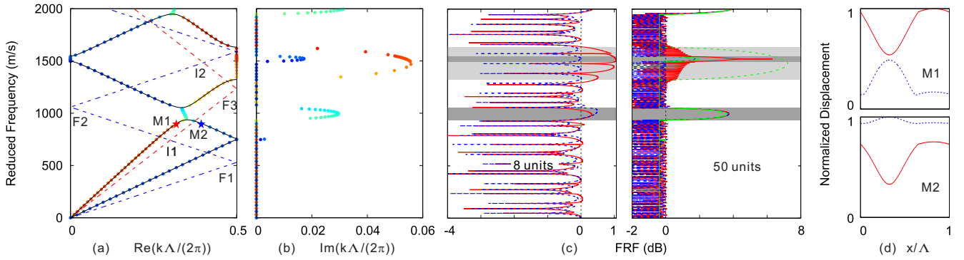
Figure 5: Complex band structures for 1D lossless FSPM with periodic layers of FSP medium. Panels (a) and (b) illustrate the variation of the reduced frequency with the real and imaginary part of the wave vector, respectively. The solid lines represent the real band structures obtained by using Eqs. (13) and (15). The blue and red dashed lines are the dispersion curves of P1 and P2 waves for lossless FSP media, as obtained by Eq. (17). The colorscale is the same as that in Fig. 2. FRF curves of a finite metamaterial with 8 or 50 unit cells are shown in panel (c). The solid and dashed lines represent the results for the excitation of P1 and P2 waves, respectively. The light gray region indicates the Bragg bandgap for P1 wave in panel (a), while the gray regions show the complete bandgaps for both P1 and P2 waves. The green lines represent the results predicted by using Eq. (19) through the imaginary part of the wave vector for P1 wave (dashed lines for P2 wave). Normalized displacement distributions at the marked points in panel (a) are illustrated in panel (d). The relative energy ratio is 0.74 at point M1 and 0.27 at point M2.
