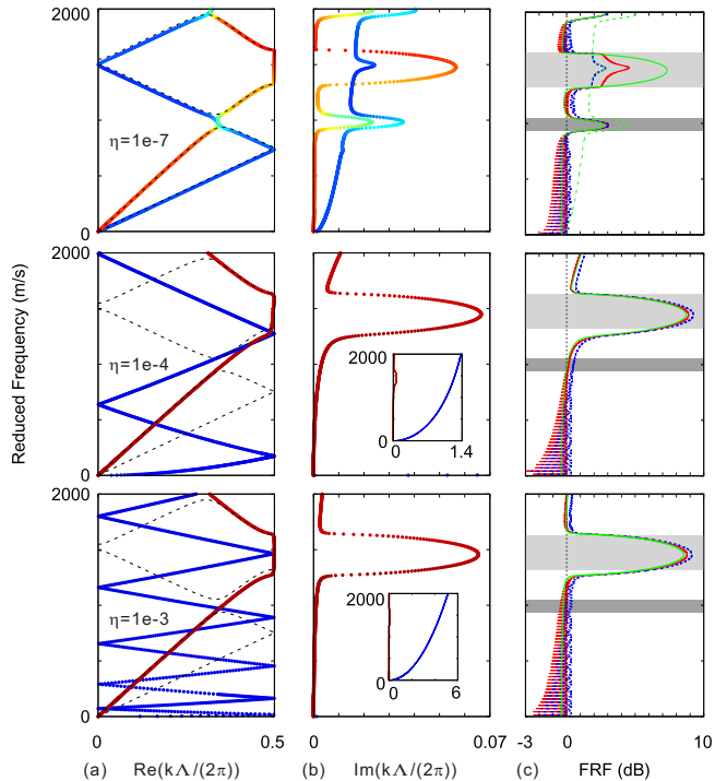
Figure 6: Influence of fluid viscosity on complex band structures for 1D FSP metamaterials. Panels (a) and (b) show the variation of the reduced frequency with the real and imaginary part of the reduced wavenumber. The colorscale is the same as that in Fig. 2. The insets in (b) show a larger view of the imaginary part of the wavenumber. The attenuation properties of a finite metamaterial with 50 periods are shown in panel (c). The red solid and blue dashed lines represent the results for the excitation of u_x and w_x , respectively. The green lines represent the results predicted by Eq. (19) for the P1 wave (green dashed lines for the P2 wave). The gray areas indicate the bandgaps for the lossless FSPM in Fig. 5.
