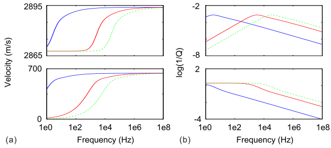
Figure 3: Variation of the phase velocity (a) and of the attenuation (b) with frequency for different viscosities of the pore fluid. The horizontal axis is shown with a logarithmic scale. The thick-solid blue, thin-solid red, and thin-dashed green lines represent the results for \eta = 10^{-7} , 10^{-4} and 10^{-3} Pa·s, respectively. The upper and lower panels present the results for P1 and P2 waves, respectively.
