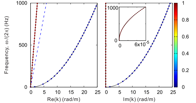
Figure 2: Complex band structures for homogeneous FSP media. The left and right panels illustrate the variation of the frequency with the real and imaginary part of the wave vector, respectively. The solid lines represent for the analytical results obtained by Eq. (17). The colorscale indicates the relative energy ratio between the solid skeleton (1) and the pore fluid (0). The blue and red dashed lines represent the analytical dispersion curves for lossless homogeneous media. The inset shows a closer view to the imaginary part at the origin.
