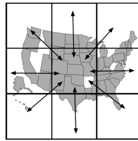
Figure 3: An example of grid decomposition on x and y axes for the platform D-Mason on nine processors [13]
