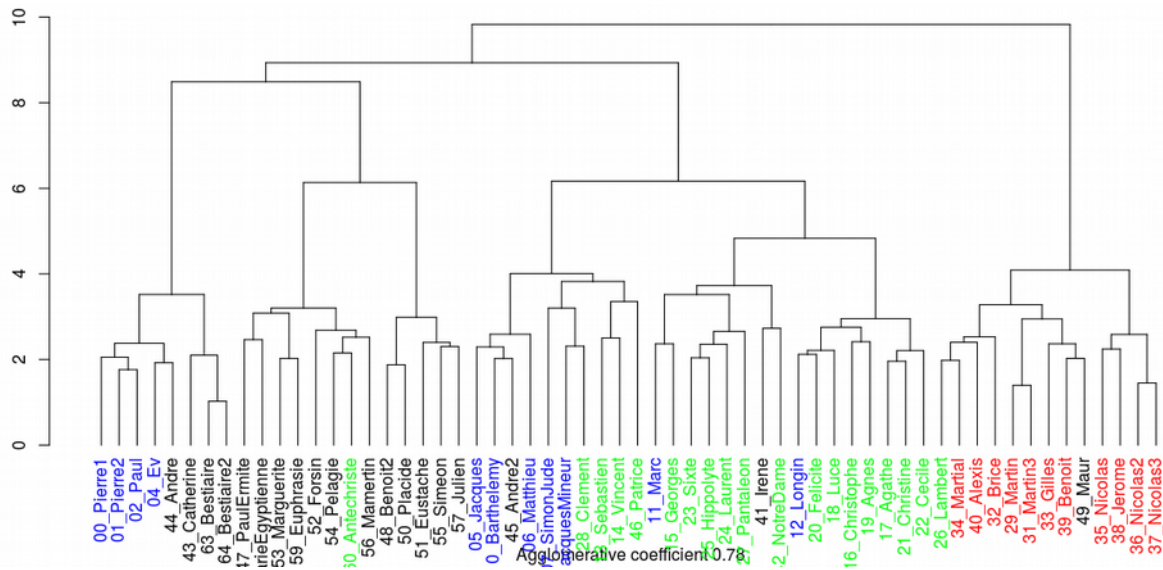
Illustration 2: Dendrogram of agglomerative hierarchical clustering using Kohonen SOM coordinates over 400 most frequent 6-grams
