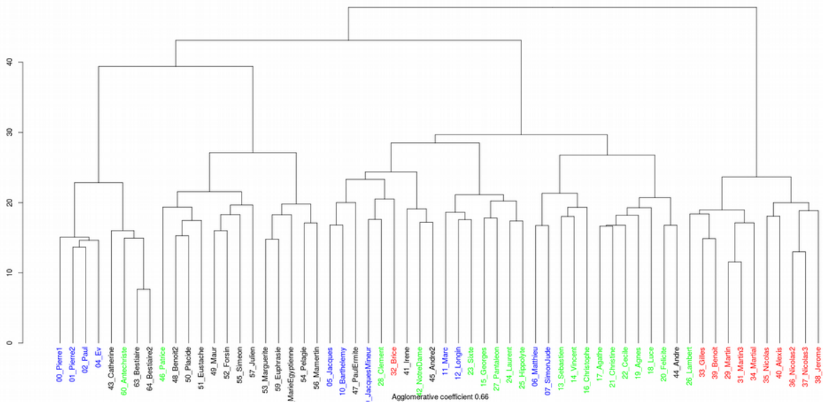
Illustration 1: Dendrogram of agglomerative hierarchical clustering using Manhattan distance, z-transformation and vector length normalization over 400 most frequent 6-grams
