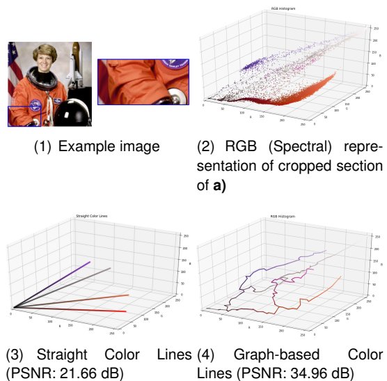
Figure 1: Comparison between SCL and GCL. Our model fits spectral representation by piecewise lines.
