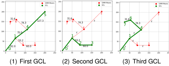
Figure 5: Illustrative example of Algorithm 1
