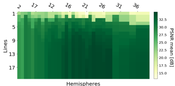
Figure 8: PSNR varying the number of GCL and hemispheres from Table 1.
