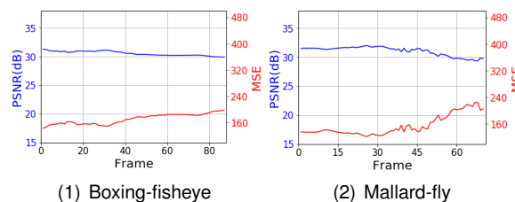
Figure 9: PSNR and MSE in two videos from (16). PSNR (blue) and MSE (red).
