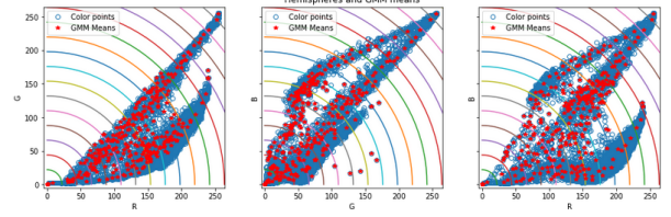
Figure 3: Gaussian means of spectral representation of cropped section Fig. 1 (a).
