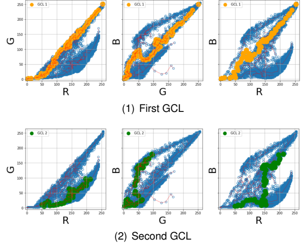
Figure 6: First two GCL of cropped section Fig. 1 (a)
