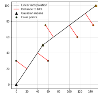
Figure 7: Illustrative example of color points projection on a GCL
