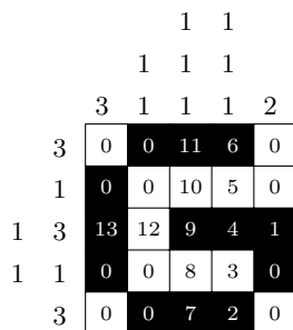
Fig. 7: Graphic representation of the decomposition obtained for the game Nonogram 5 \times 5 . The number in each cell represents the subgame to which it belongs.
