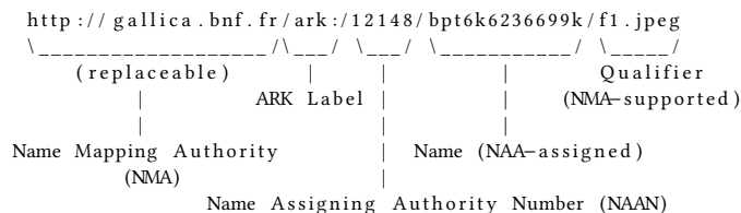
Fig. 1. Scheme of an ARK.
