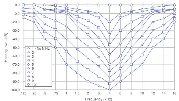
Figure 2: Audiograms used in the simulation of 10 levels NIHL, expressed in hearing loss (dB) for each frequency band (kHz).
