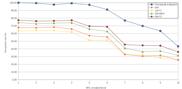
Figure 5: Perceptual and automatic recognition rate (using the different language model/lexicon configurations) per simulated NIHL degradation level for task T2 (sentences).
