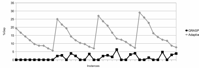
Figure 4: GRASP results on random instances with E^- \cap E^+ \neq \emptyset .
