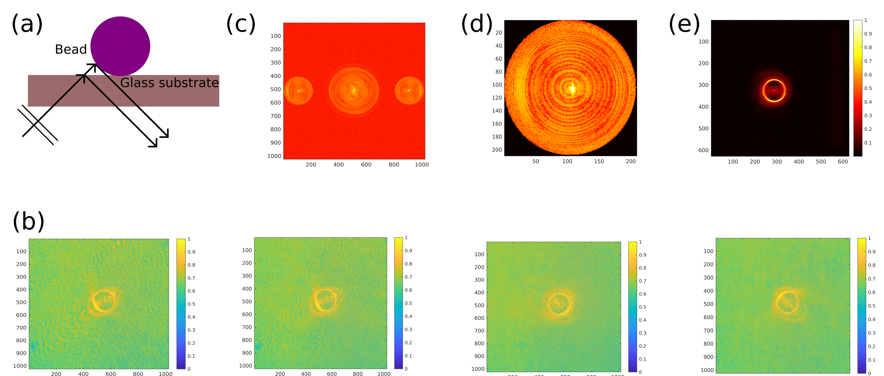
Fig. 2. (a) Bead (dia of 6 \mu m) on substrate, (b) Hologram at different illumination angle (74°, 61°, 23°, 67°). (c) The hologram in Fourier space (d) The desired order as filtered form (c). (e) The bead interface (Note: for images (b-e) both x and y axis indicates No. of pixel)
