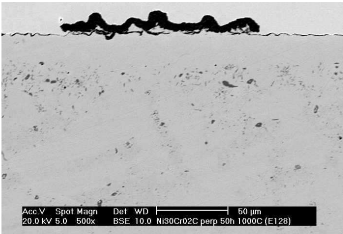
b Ni-30Cr-0.2C after 50 hours at 1000°C
