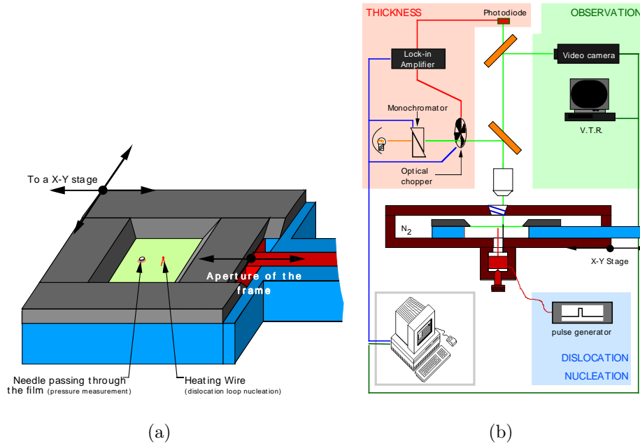
Fig. 3. (a): The schematic representation of the frame. One of its sides can be moved in order to change the aperture of the frame. The heating wire lies about 50\mu\text{m} below the film. The needle is used to create a meniscus in the film in place where it can be easily observed. The meniscus forms around the needle. (b): The schematic representation of experimental setup. The frame is placed in a temperature controlled oven. The film is observed through the reflecting microscope. The reflectivity as a function of the incident wavelength is determined with the help of a computer controlled monochromator. An optical chopper and a lock-in allow to exclude parasitic light.
