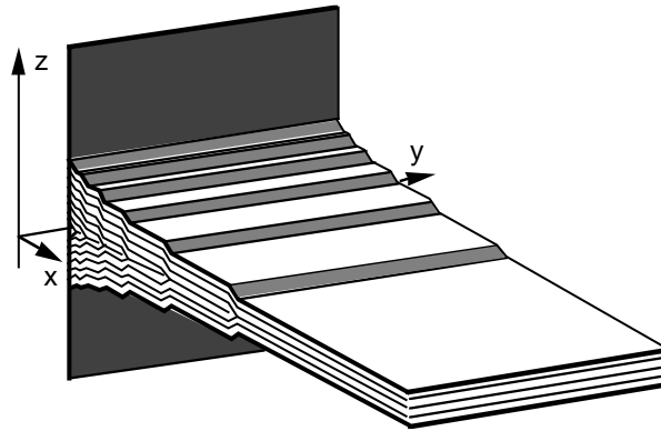
Fig. 2. The schematic and idealized picture of the smectic meniscus close to the wall (after Ref. [5]). The dislocations are stabilized in the mid-plane due to the repulsion from the two free surface shown in the picture.
