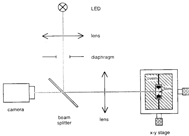
FIG. 2. Experimental setup.
