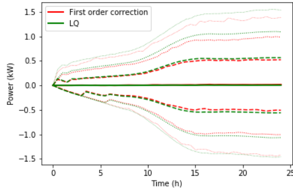
Figure 4: Time evolution of quantiles of deviations p^{\text{grid}} - \mathbb{E}[p^{\text{grid}}]
