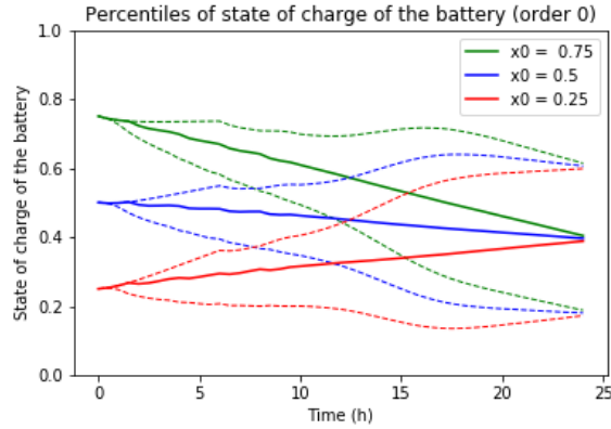
Figure 6: Time evolution of the empirical quantiles 95%, 50%, 5% of the state of charge of the storage system
