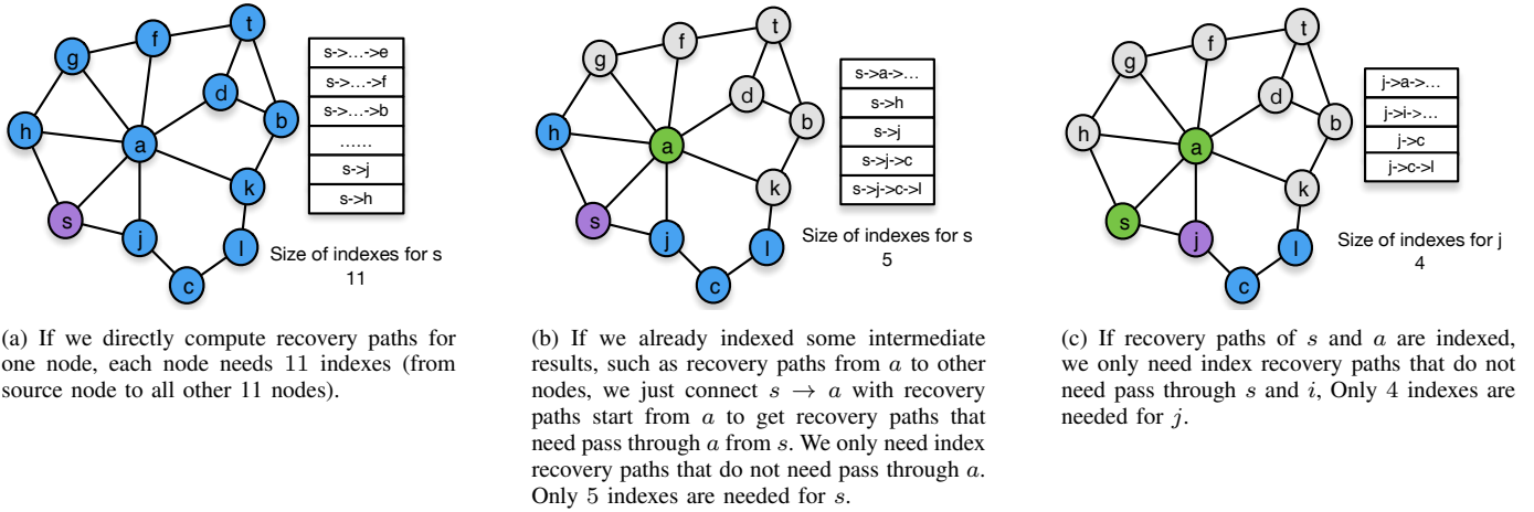
Fig. 3. The differences in index size between the naive method (a) and our method (b) (c).
