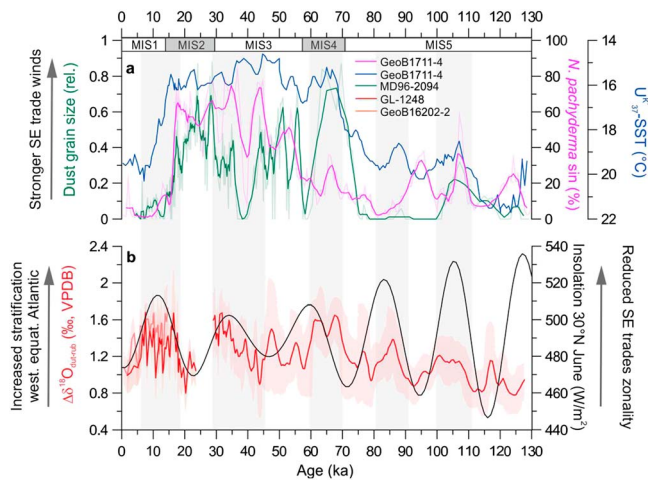
Figure 9. Upper ocean stratification in the western equatorial Atlantic compared to trade wind strength and zonal for the last 130 ka. (a) Proxies from the subtropical South Atlantic near the Benguela upwelling system (Figure 1b) linked to southeast trade wind intensity. Relative abundance of N. pachyderma (sinistral) from core GeoB1711-4 (Little et al., 1997; pink line) with a 5-point running average (thick pink line). Relative abundance of coarse-grained dust to total windblown dust from core MD96-2094 (Stuut et al., 2002; green line) with a 5-point running average (thick green line). Alkenone-based sea surface temperatures from core GeoB1711-4 (Kirst et al., 1999; blue line). (b) Our Monte Carlo ensemble \Delta\delta^{18}\text{O}_{\text{dut-rub}} mean values from cores GeoB16202-2 (red line) and GL-1248 (red line for the lower part and light red line for the upper part of the record). Shadings with the same color code indicate the 95% confidence envelope including age and analytical uncertainties. Mid-June 30°N insolation (solid gray line) are displayed (Berger & Loutre, 1991). Marine isotope stages (MIS) are highlighted below the upper x-axis. Gray bars highlight key periods of increased stratification on our \Delta\delta^{18}\text{O}_{\text{dut-rub}} records (GL-1248 and GeoB16202-2) and increased mid-June 30°N insolation.
