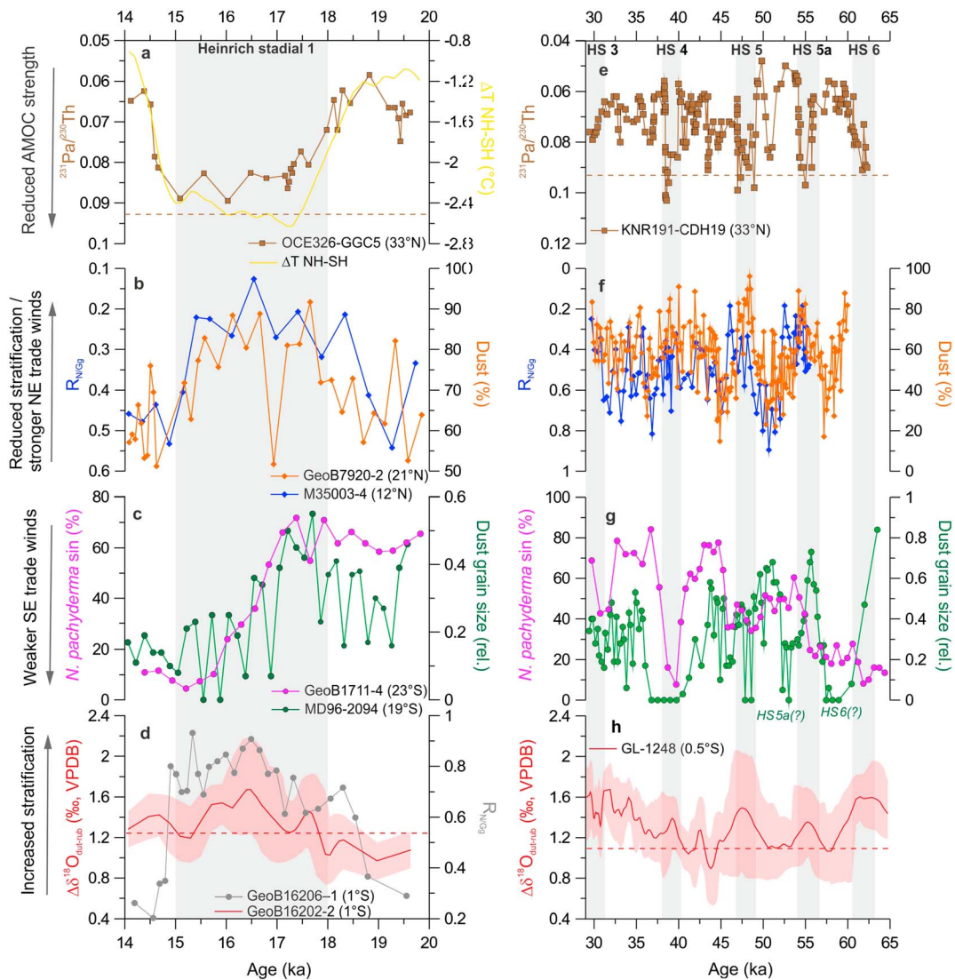
Figure 8. Upper ocean stratification in the western equatorial Atlantic during Heinrich stadials compared to other proxies. (a) ^{231}Pa/^{230}Th records from core OCE326-GGC5 from the Bermuda rise (McManus et al., 2004; brown line and squares) and reconstruction of hemispheric surface temperature difference (Shakun et al., 2012; yellow line). The brown dotted line represents the ^{231}Pa/^{230}Th production ratio of 0.093, which indicates sluggish or absent overturning circulation. (b) Stratification proxy from the western tropical North Atlantic and a dust record from the eastern tropical North Atlantic. The R_{N/Gg} ratio (% Neogloboquadrina / (% Neogloboquadrina + % G. glutinata )) from core M35003-4 (Hüls & Zahn, 2000; Portilho-Ramos et al., 2017; blue line and diamonds) in the western tropical North Atlantic. Relative percentage of dust from core GeoB7920-2 (Collins et al., 2013; orange line and diamonds) in the eastern tropical North Atlantic. (c) Proxies from the subtropical South Atlantic near the Benguela upwelling system (Figure 1b) linked to southeast trade wind intensity. Relative abundance of Neogloboquadrina pachyderma (sinistral) from core GeoB1711-4 (Little et al., 1997; pink line and circles). Relative abundance of coarse-grained dust to total windblown dust from core MD96-2094 (Stuut et al., 2002; green line and circles). (d) Proxies for stratification in the western equatorial Atlantic. The R_{N/Gg} ratio (% Neogloboquadrina / (% Neogloboquadrina + % G. glutinata )) from core GeoB16206-1 (Portilho-Ramos et al., 2017; gray line and circles) and the Monte Carlo ensemble \Delta\delta^{18}O_{dut-rub} mean values from core GeoB16202-2 (this study; red line). Red shading indicates the 95% confidence envelope including age and analytical uncertainties. The red dotted line represents the \Delta\delta^{18}O_{dut-rub} core top value from GeoB16202-2. The gray bar marks the time interval of Heinrich stadial 1 (18–15 ka). (e) ^{231}Pa/^{230}Th records from core KNR191-CDH19 also from the Bermuda rise (Henry et al., 2016; brown line and squares). The brown dotted line represents the ^{231}Pa/^{230}Th production ratio of 0.093. (e) Same records as in (b). (f) Same records as in (c). (g) The Monte Carlo ensemble \Delta\delta^{18}O_{dut-rub} mean values from core GL-1248 (red line), with the red 95% confidence envelope (red shading). The red dotted line represents the \Delta\delta^{18}O_{dut-rub} core top value from GL-1248. Gray bars highlight the Heinrich stadials (HS3, HS4, HS5, HS5a, and HS6). Note that the published records presented here are shown on their original chronologies.
