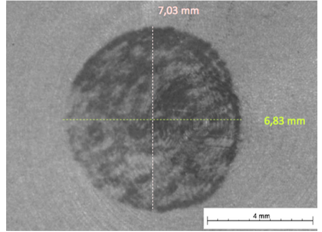
FIG. 11. 0.377\ \text{cm}^2 target illumination spot. Photo of the Delrin (POM) target after metallization with 7 nm Pt.
