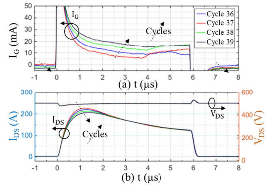
Fig. 3. Permanent degradation of the gate during repetitive SC operations. Evolution of (a) I_{\text{G}} and (b) V_{\text{DS}} and I_{\text{D}} during short-circuit. Each color represents a SC. ( V_{\text{DS}} = 500\text{V} ; V_{\text{driver}} = 21\text{V}/-5\text{V} ; T_{\text{case}} = 25^\circ\text{C} ; R_{\text{G}} = 100\Omega ).
