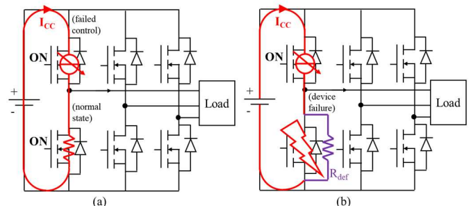
Fig. 1. Inverter-leg shoot-through operation : (a) by control signals. (b) by electrical breakdown of one of the power devices.
