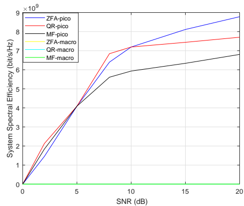
Figure 4. System spectral efficiency bit/s/Hz for macro & pico cells.
