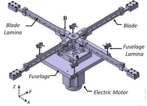
Fig. 2 The final design of the experimental helicopter for ground resonance analysis
