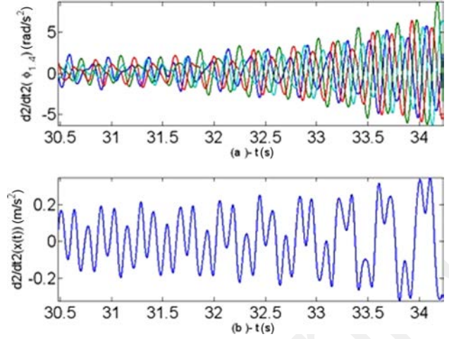
Fig. 6 Time history of the experimental helicopter with IR configuration at \Omega \approx 7.5 Hz; (a) blades and (b) fuselage accelerations
