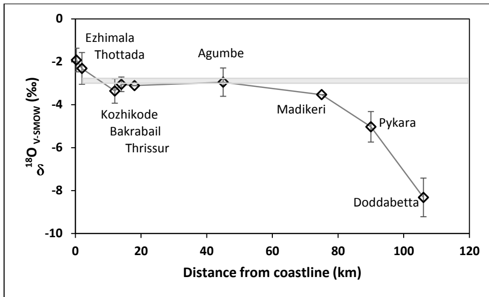
67 Fig. 5: The variability of oxygen isotope ratio ( \delta^{18}\text{O} ) for nine major sampling locations as a 68 function of their distance to the Arabian Sea coast. The grey box corresponds to the mean 69 oxygen isotope ratio ( \delta^{18}\text{O} = -3.1 \pm 0.3\text{‰} ; Tripti et al. 2016) of groundwater in southwest 70 coast of India.
