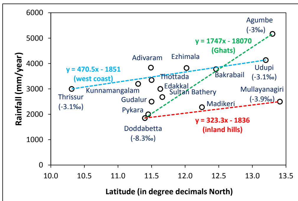
1 2 Fig. 1.d.: Rainfall variability (rainfall amount data from www.worldweatheronline.com and 3 corresponding station spring/groundwater isotope ratio from our study) along the west coast 4 and inland regions adjacent to the Western Ghats, South India.
