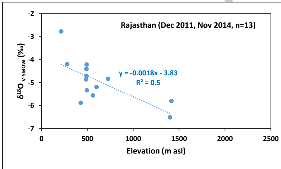
105 Fig. 7: Plot showing relationship between elevation and oxygen isotope ratio ( \delta^{18}\text{O} ) for 106 groundwater in Sri Lanka (July 2012) and Rajasthan (December 2011 and November 2014), 107 India (data from Lambs, under preparation).
