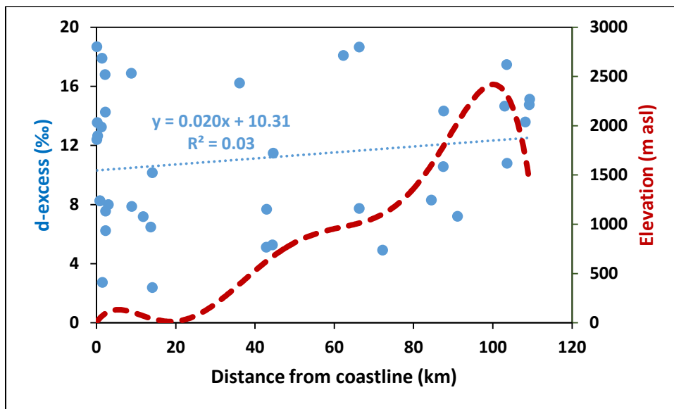
116 Fig. 8: The variability of deuterium-excess in the sampled water (lake, pond and bore well 117 samples are not included to avoid any effect from evaporation) along the Western Ghats and 118 its adjacent slopes during this study. Note that water from the mountains close to the west 119 coast of India exhibit higher d-excess range between 3 ‰ and 20 ‰ whereas lower variability 120 is observed in inland region corresponding to highest elevations in the Western Ghats 121 monitored during this study.
