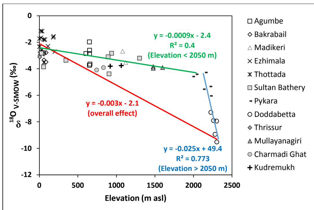
50 Fig. 4: Relationship between elevation and oxygen isotope ratio ( \delta^{18}\text{O} ) along the mountain 51 belt of the Western Ghats. The first regression line in green colour is for the stations below 52 2050 m asl and the second line in blue is for the stations beyond 2050 m asl in the Nilgiri 53 ranges. The overall slope of 0.31 ‰/100 m for the isotope ratios of water from the west coast 54 to the highest elevation (sampled here at 2300 m asl) of the Western Ghats is given in red to 55 compare with the reported global isotopic lapse rate (0.28 ‰/100 m; Poage and Chamberlain, 56 2001). Note the data for Mullayanagiri - Charmadi Ghat (Lambs et al. 2011) and Kudremukh 57 (Tripti et al. 2016) are from published work.
