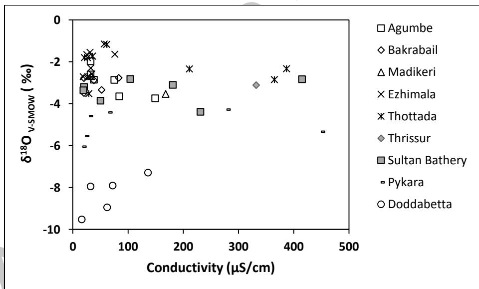
25 Fig. 2.b.: Relationship between conductivity and oxygen isotope ratio ( \delta^{18}\text{O} ) for the 26 November/December 2013 water samples (Agumbe, Bakrabail, Pykara, Doddabetta, Sultan 27 Bathery and Thrissur) and the October 2014 water samples (Ezhimala and Thottada).
