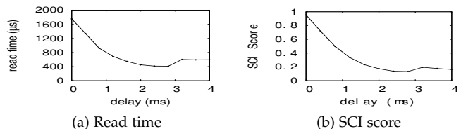
Fig. 6: I/O contention micro-benchmark
