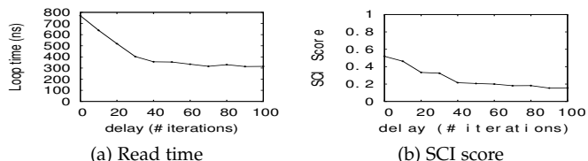
Fig. 5: False-sharing micro-benchmark
