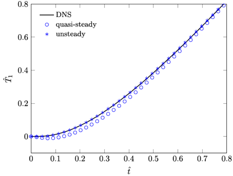
Fig. 7. Comparison between the unsteady/quasi-steady models and the reference solution obtained by averaging Direct Numerical Simulations (DNS) results of the micro-scale problem.
