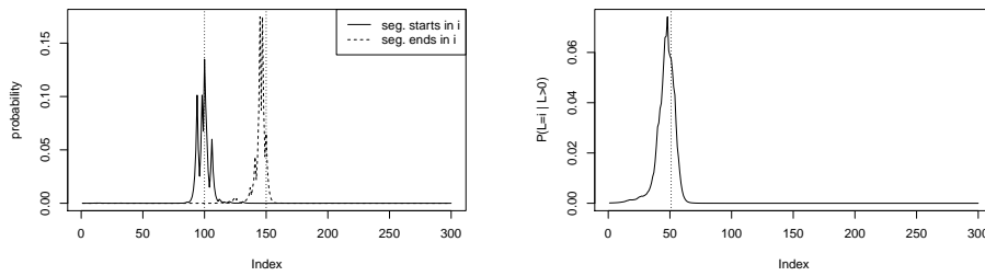
Fig. 4 Segment start/end posterior distribution (left Panel) and length (right Panel) for the simple simulation with n = 300 and I = [100, 150] , q_0 = (0.4, 0.2, 0.2, 0.2) , q_1 = (0.2, 0.4, 0.3, 0.1) and f = \log(q_0/q_1) .
