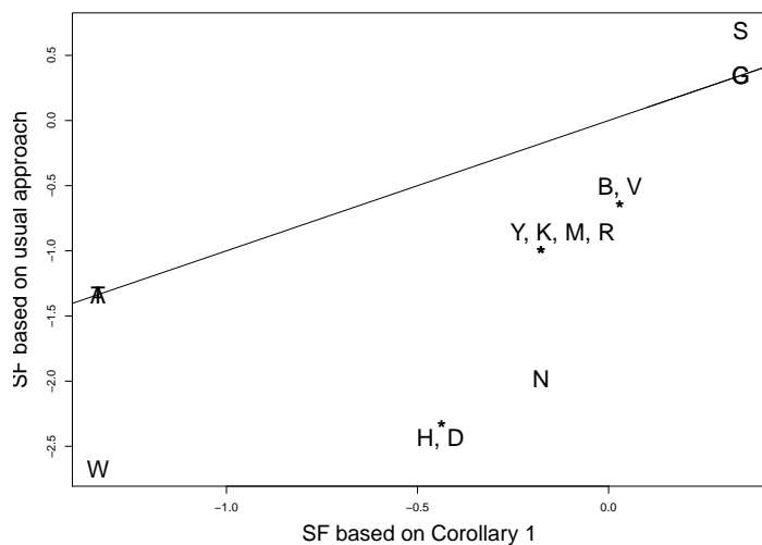
Fig. 7 Scoring function (SF) \sigma using Theorem 1 for A, C, G, T and Corollary 1 for the ambiguous components, and \tilde{\sigma} using Theorem 1 for A, C, G, T and the usual approach for the other components.
