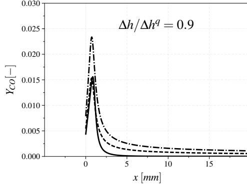
Figure 4: CO mass fractions profiles computed for a burner stabilized flame at \phi = 0.8 and at fixed \Delta h/\Delta h^q . Continuous line: Detailed chemistry calculations. Dashed dot line: Adiabatic virtual chemistry calculation. Dashed line: Non adiabatic virtual chemistry calculations.
