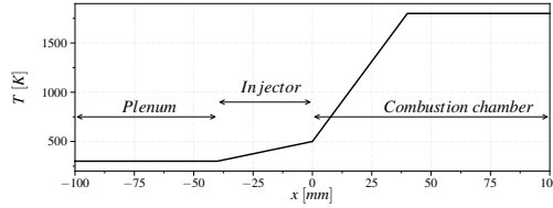
Figure 6: Wall temperature profiles imposed along the flame side wall chamber [41].
