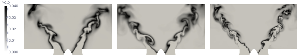
Figure 9: Instantaneous CO filtered mass fraction snapshot on the middle-plane of the combustion chamber. From left to right: AC, NAC, NAF.
