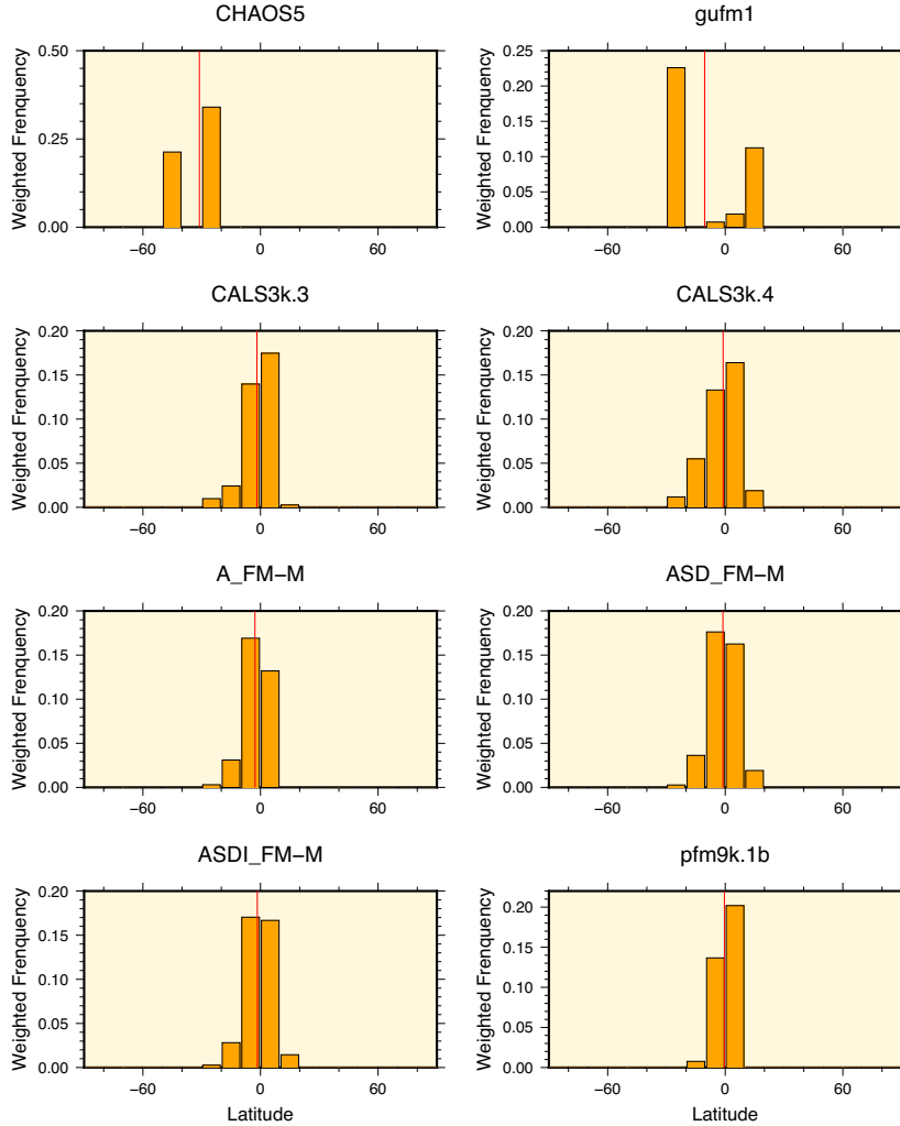
Figure 6. As in Fig. 5 for latitude. Weighted frequency is the integral over time of W_{\theta}() . Red vertical lines denote persistent peaks (15).
