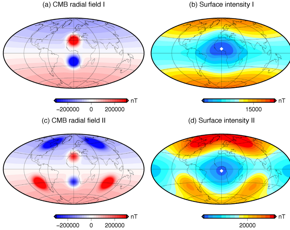
Figure 3. Synthetic radial field models at the CMB (a, c) and their corresponding surface intensities (b, d). In (a) the RFPs are at 30°N and 20°S. In (c) the NFPs are at 60°N and 30°S and the RFPs are at 30°S and 30°N. White diamonds in (b) and (d) indicate local surface intensity minima. The minima latitudes are 10°N and 4°S in (b) and (d), respectively.
