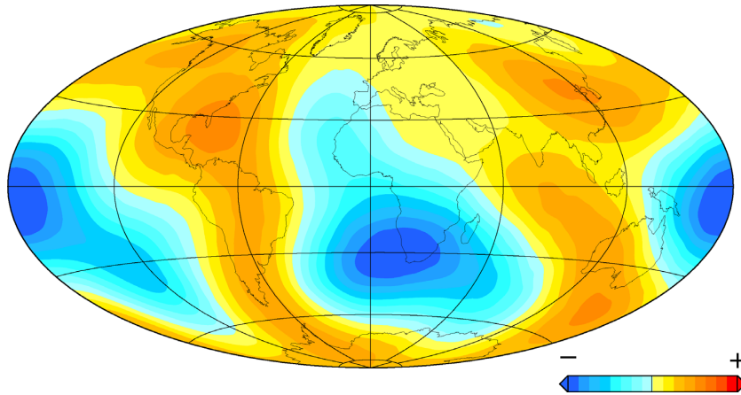
Figure 2. Heterogeneous heat flux anomalies based on tomographic seismic shear wave anomalies at the lowermost mantle (Masters et al. 2000) truncated at spherical harmonic degree 6. This pattern was imposed as a heterogeneous outer boundary heat flux in the dynamo models. Red/blue corresponds to large/low heat flux (and thus colder/hotter mantle), respectively.
