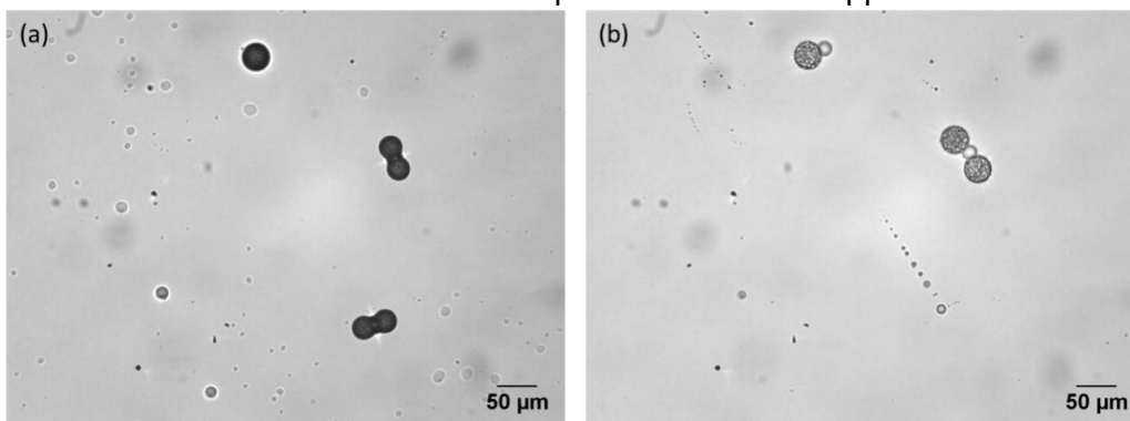
Figure 8: Images of (a) dried Na-alginate microparticles and (b) Ca-alginate microparticles after immersion in CaCl_2 solution (0.5wt%). Experimental conditions: C_i = 0.25wt\% , DMC flowrate = 0.05\mu l/s and k=5 .
