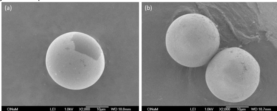
Figure 9: SEM photographs of (a) Na-alginate and (b) Ca-alginate microparticles (formed in a 0.5wt% CaCl 2 solution). (Same experimental conditions as for Figure 8)
