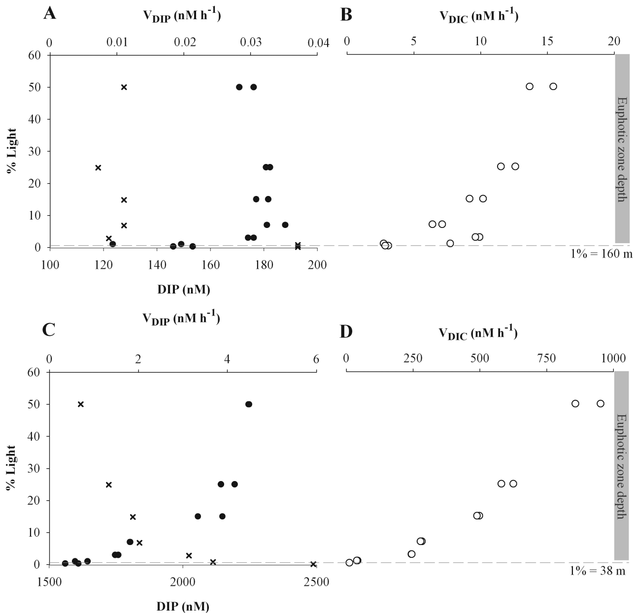
Fig. 4. DIP (●), DIC uptake rates (○) (nM h -1 ) (duplicates), and DIP concentrations (x) (nM) in the south Pacific gyre (A and B) and in the Chilean upwelling (C and D). The data are presented according to the in situ light levels (%). The 1% depth is indicated by a gray dotted line.
