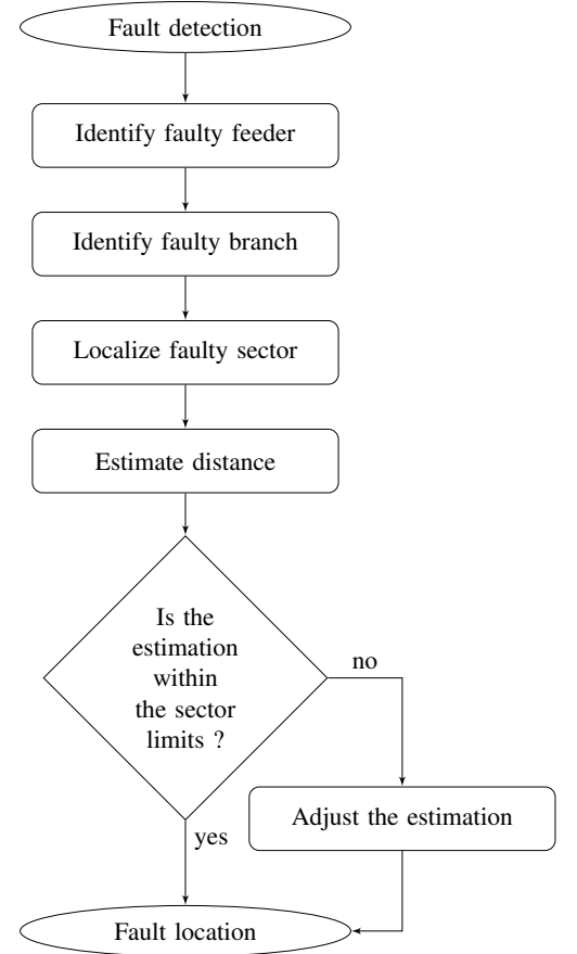
Fig. 3: Fault localization method flowchart
