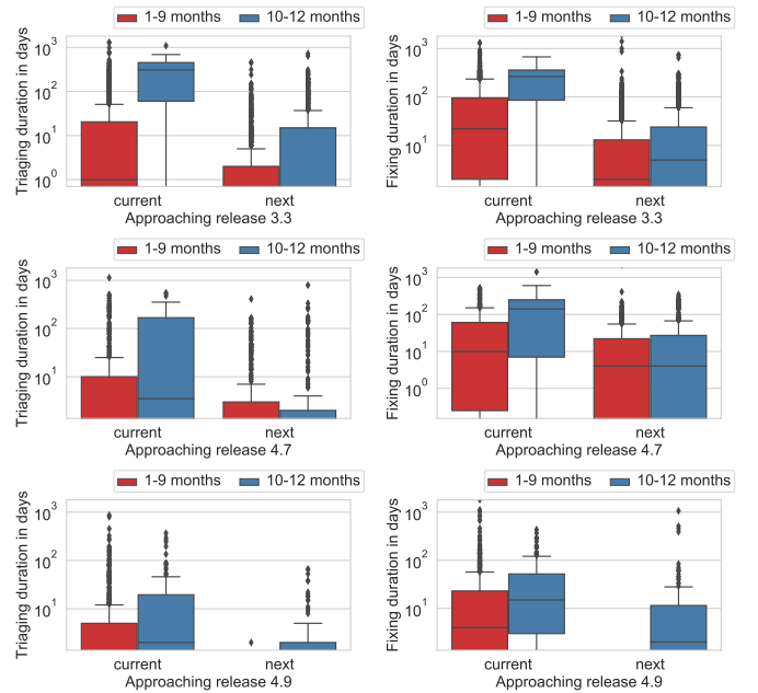
Fig. 8: Triaging time distributions (left figures) and fixing time distributions (right) when approaching next release.
