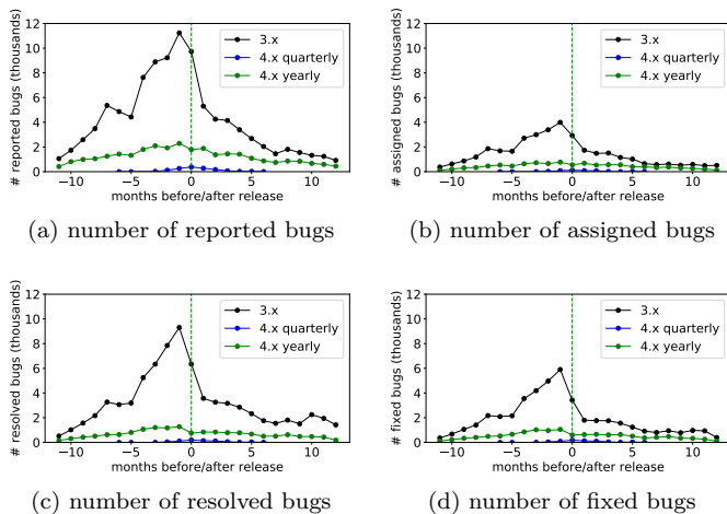
Fig. 5: Monthly evolution of the number of bugs before/after a release, aggregated by release series (y-axis is measured in thousands of bugs).
