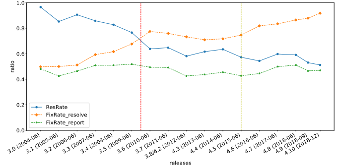
Fig. 3: Resolution and fixing rates per targeted Eclipse release.
