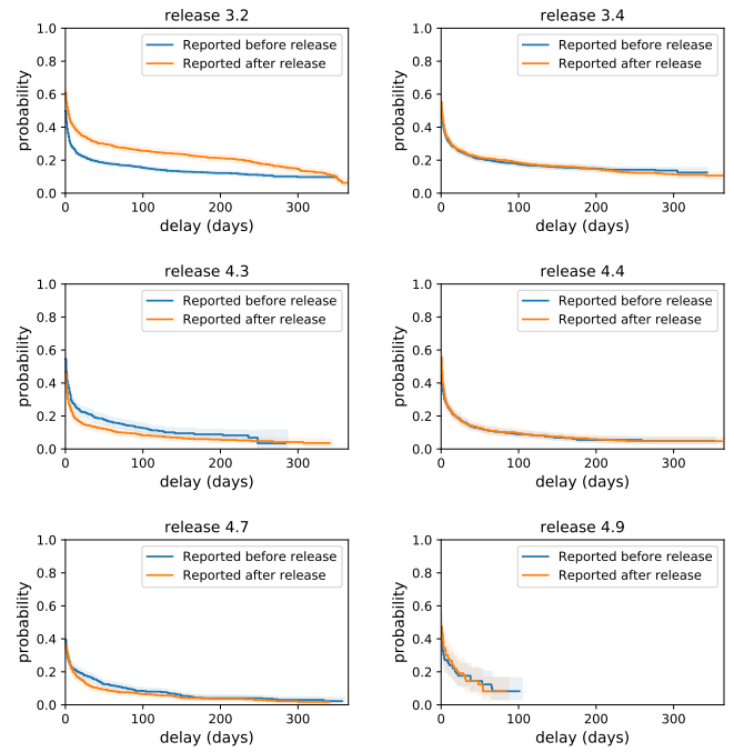
Fig. 7: Kaplan-Meier survival curve with 95% confidence interval (indicated by the shaded areas) for triaging time before and after each release.
