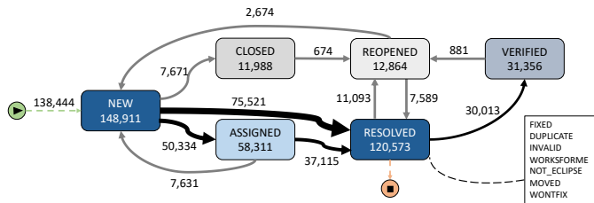
Fig. 1: The life-cycle of Eclipse bug reports.
