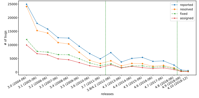
Fig. 2: Number of bugs targeting a specific release. The vertical dashed lines indicate the switch from Eclipse 3.x to 4.x, and from an annual to a quarterly cycle after 4.8.
