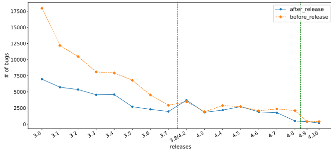
Fig. 4: Reported bugs before and after each release.
