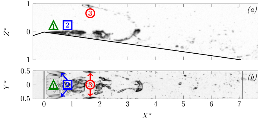
FIG. 4. Side (a) and top (b) views of typical transitioning flow, with attached cavities and vaporisation of a hairpin vortex, captured at Re = 2185 and \sigma = 4.53 . The flow is from left to right. The two black lines positioned at X^* = 0 and X^* = 7.1 indicate respectively the throat and the end of the Venturi slope. The different attached cavities usually observed into laminar separated flows, namely the “band” cavity, the “tadpole” cavities and the secondary “tadpole” bubbles, are respectively associated with a symbol ( \triangle , \square and \circ ) and numbered from 1 to 3.
