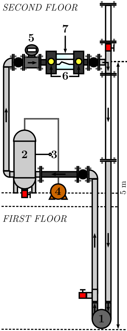
FIG. 3. Sketch of the test loop with (1) the pump, (2) the oil tank, (3) the temperature sensor, (4) the compressor or vacuum pump, (5) the ultrasonic flowmeter, (6) the pressure sensors and (7) the operating test section detailed in figure 2.
