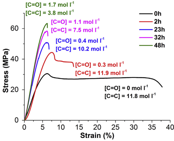
Fig. 12. Tensile curves for PDPCD samples with varying exposure times at 80 °C under air. NB: Concentrations were obtained by using a correction corresponding to \left(\frac{\Delta_{ox}}{e}\right) differences in samples tested for tensile tests and ageing tests monitored by FTIR.
