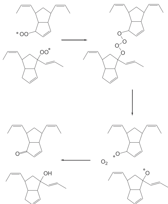
Scheme 4. Termination step: Russell disproportionation of PO^\circ .
