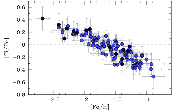
Fig. 10. Titanium abundances in Sculptor. Stars overlapping with the sample from Hill et al. (in prep.) are blue, while stars observed here for the first time with HR spectra are dark blue.
