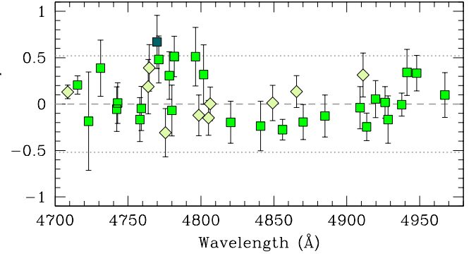
Fig. 6. Average deviation of the measured Ti lines from the mean, as a function of wavelength, equivalent to Fig. 4. Green squares are Ti I lines, pale green diamonds are Ti II lines and the dark green square is a Ti I line falling out of the criteria. The bluest part of the spectrum ( <4740 \text{ \AA} ) is only usable for the brightest stars, so these points and their standard deviations are determined from measurements in \leq 6 stars.
