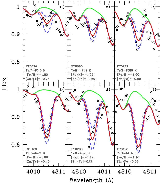
Fig. 12. Zn I line at 4810.5 Å for three pairs of stars with similar stellar parameters but very different [Zn/Fe] values: a ) and b ) show stars with [Fe/H] \approx -1.8 ; c ) and d ) stars with [Fe/H] \approx -1.5 ; e ) and f ) stars with [Fe/H] \approx -1.1 . In each case, the spectrum is shown with black crosses, while the best fit is shown with a red solid line, and blue dashed lines show upper and lower errorbars (including error due to stellar parameters). The green solid line shows the case where there is no Zn present.
