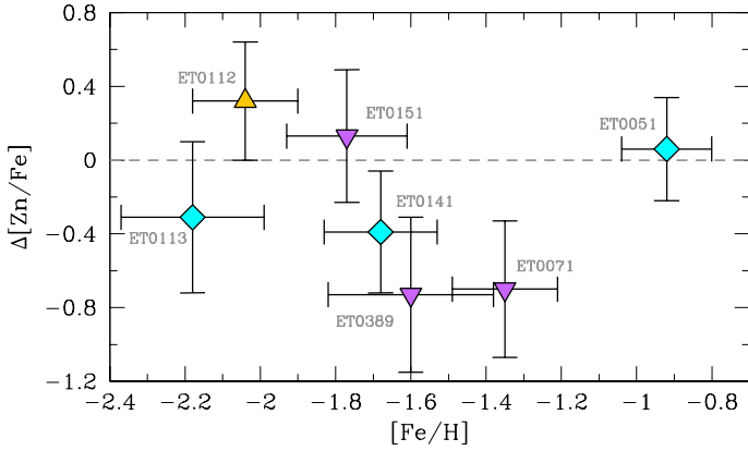
Fig. 9. Difference between [Zn/Fe] measurements from seven stars in this work and the literature. Downward pointing violet triangles are stars from Shetrone et al. (2003), and cyan diamonds from Geisler et al. (2005), both using UVES slit spectra. The orange triangle is a star measured by Hill et al. (in prep.) with FLAMES/UVES spectra.
