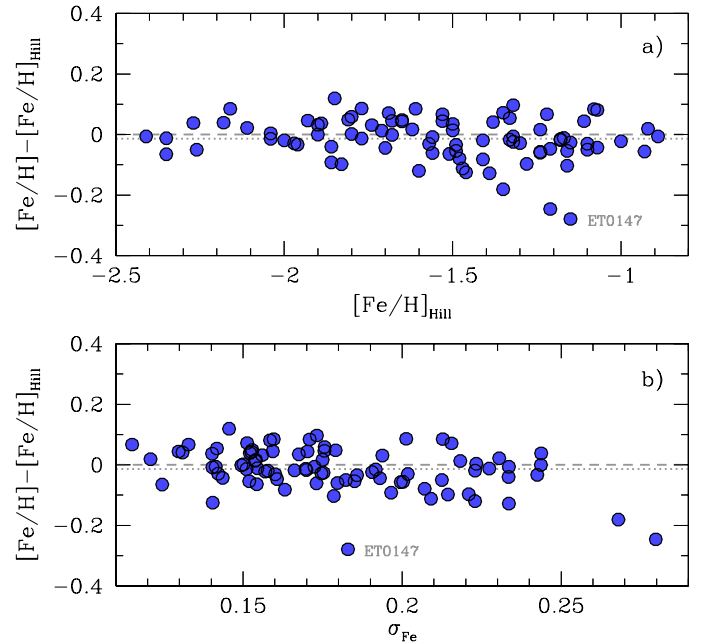
Fig. 5. Difference between [\text{Fe}/\text{H}] measurements from this work, and Hill et al. (in prep.) as a function of: a) [\text{Fe}/\text{H}]_{\text{Hill}} ; b) the scatter among Fe lines, \sigma_{\text{Fe}} , as measured here. The dotted line shows the average difference between the two measurements.
