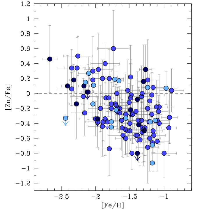
Fig. 11. Relation between [Zn/Fe] and [Fe/H] . Symbols are the same as in Fig. 10 with light blue circles showing results from the literature, using HR UVES data (Shetrone et al. 2003; Geisler et al. 2005; Jablonka et al. 2015; Hill et al., in prep.), excluding stars overlapping with the FLAMES sample. Upper limits where [Zn/Fe] > 0.6 are not included.
