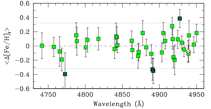
Fig. 4. Average deviation of the measured Fe lines from the mean, as a function of wavelength. The standard deviation of the sample of stars is shown by an errorbar. The dotted lines show the 2\sigma interval of the scatter. Green squares are Fe I lines, while the one available Fe II line is a pale green diamond. Dark green squares are Fe I lines that deviate more than 2\sigma from the mean. We note that a different number of measurements goes into each point, depending on the number of stars in which the line could be measured.
