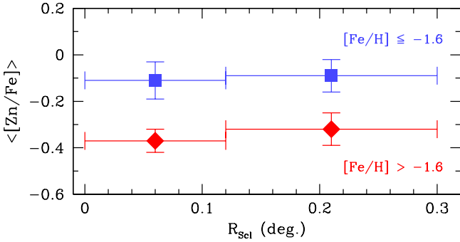
Fig. 14. Average abundance ratios of [Zn/Fe] as a function of distance from the centre of Sculptor, R_{scl} , separated by metallicity. Blue squares are stars with [Fe/H] \leq -1.6 and red diamonds have [Fe/H] > -1.6 . The x -errorbars show the size of the bins, and y -errorbars the error of the mean.
