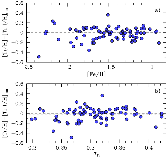
Fig. 7. Difference between [\text{Ti}/\text{H}] from this work, and [\text{Ti I}/\text{H}]_{\text{Hill}} from Hill et al. (in prep.) as a function of: a ) [\text{Fe}/\text{H}] ; b ) the standard deviation between lines, \sigma_{\text{Ti}} , measured here. The dotted lines show the average difference between the two measurements.
