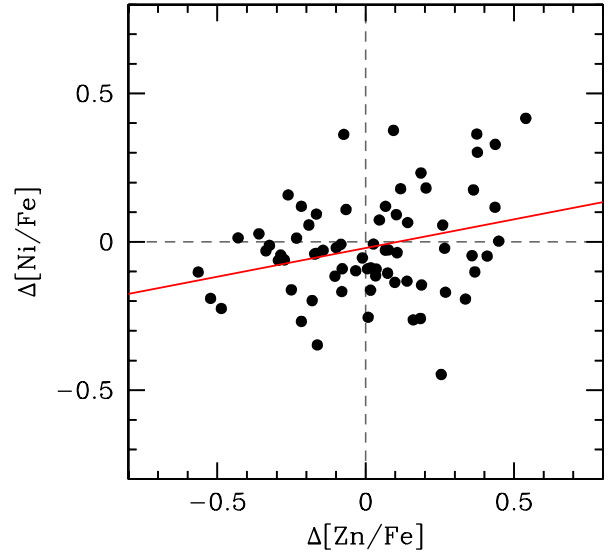
Fig. 15. Scatter of Ni, \Delta[Ni/Fe] , as a function of the scatter of Zn, \Delta[Zn/Fe] . Red line shows best fit through the measurements.
