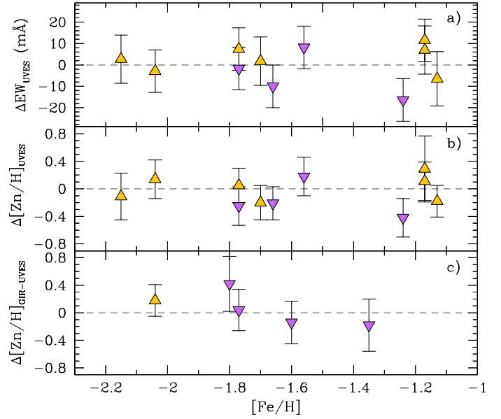
Fig. 8. Comparison of our Zn measurements with those from the literature. Errorbars show the combined uncertainties of both measurements. Downward pointing violet triangles are stars from Shetrone et al. (2003) and orange triangles are stars from Hill et al. (in prep.). The panels show differences of: a ) the measured EW of the Zn line at 4810.5 Å, between the literature and this work, in all cases using the same UVES spectra; b ) the [\text{Zn}/\text{Fe}] measurements, between the literature and this work, in all cases using the same UVES spectra; c ) the [\text{Zn}/\text{Fe}] measurements from the GIRAFFE HR7A and UVES spectra, as measured by this work.
