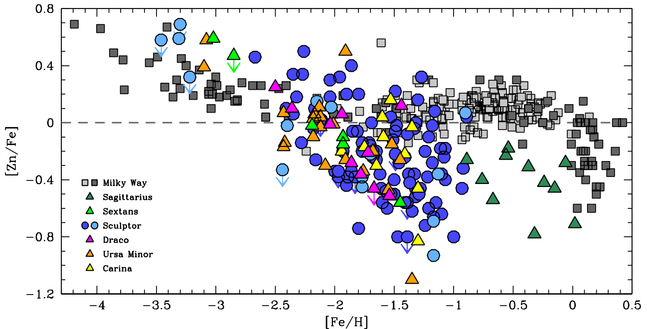
Fig. 16. Measurements of [Zn/Fe] in individual stars in the Local Group. Upper limits larger than [Zn/Fe] = 0.7 are excluded from the plot, as are stars with errors \delta_{[Zn/Fe]} > 0.5 . Blue circles show stars from this work on the Sculptor dSph, and light blue circles are Sculptor stars from the literature. Triangles are stars from other dwarf galaxies; included are (from highest to lowest stellar mass according to McConnachie 2012 ): Sagittarius stars are dark green, Sextans is green, Draco is magenta, Ursa Minor is orange, and yellow is for Carina stars. Squares are Milky Way stars, where giant stars are dark gray and dwarf stars light gray. References (Number of stars): Sagittarius : Sbordone et al. (2007) (11). Sextans : Shetrone et al. (2001) (5); Honda et al. (2011) (1). Sculptor : Shetrone et al. (2003) (1); Geisler et al. (2005) (1); Kirby & Cohen (2012) (1); Jablonka et al. (2015) (4 upper limits); Skúladóttir et al. (2015b) (1); Simon et al. (2015) (1); Hill et al. (in prep.) (6). Draco : Shetrone et al. (2001) (5); Cohen & Huang (2009) (5). Ursa Minor : Shetrone et al. (2001) (6); Sadakane et al. (2004) (3); Cohen & Huang (2010) (10); Ural et al. (2015) (2). Carina : Shetrone et al. (2003) (5); Venn et al. (2012) (5). Milky Way : Reddy et al. (2003, 2006) ; Cayrel et al. (2004) ; Nissen & Schuster (2011) ; Ishigaki et al. (2013) ; Bensby et al. (2014) (only including stars with errors \delta_{[Zn/Fe]} \leq 0.2 ); Barbuy et al. (2015) .
