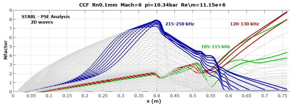
Fig. 26 STABL N factors corresponding to BAM6QT quiet run at 150 psia
