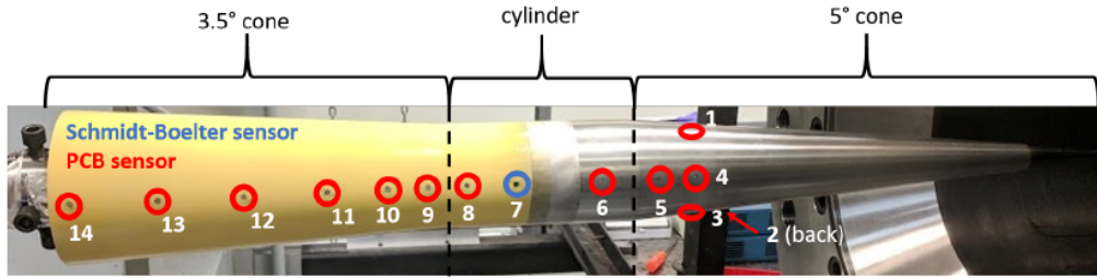
Fig. 20 Purdue model with 9 PCB sensors for BAM6QT experiments
