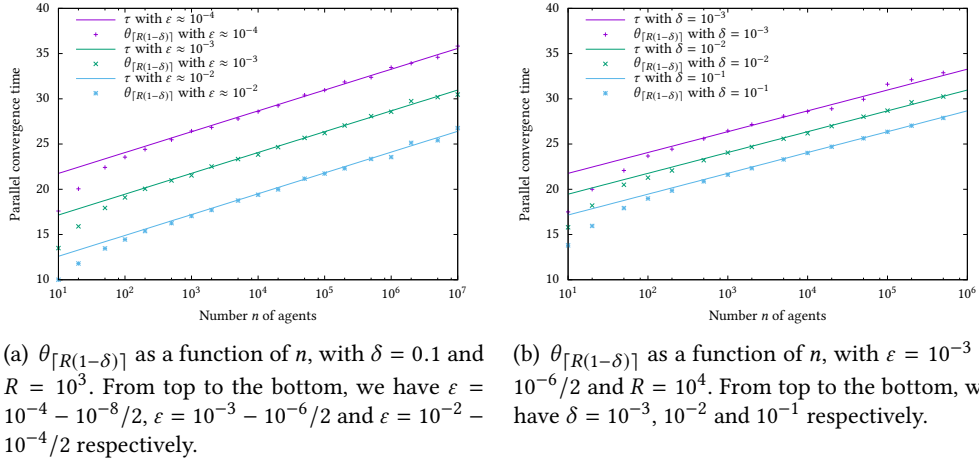
Fig. 2. Comparing the estimation \theta_{\lceil R(1-\delta) \rceil} of T with the theoretical bound \tau as a function of n .
