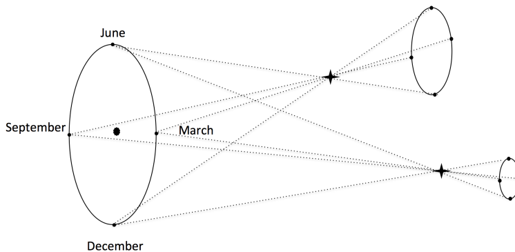
Figure 2: The parallactic motion for a nearby and a distant star.
