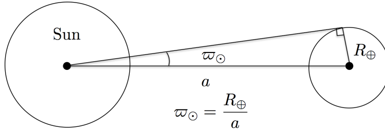
Figure 1: Definition of the solar parallax
