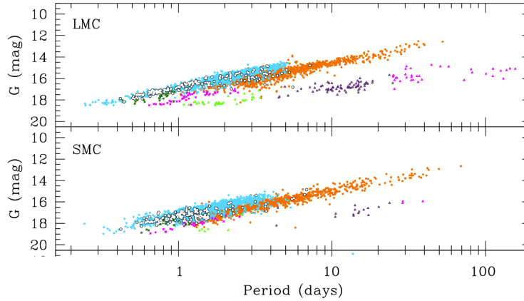
Figure 5: Period-Luminosity relation in apparent G magnitude uncorrected from reddening in the LMC and SMC from the Gaia DR2 sample (adapted from [34])
