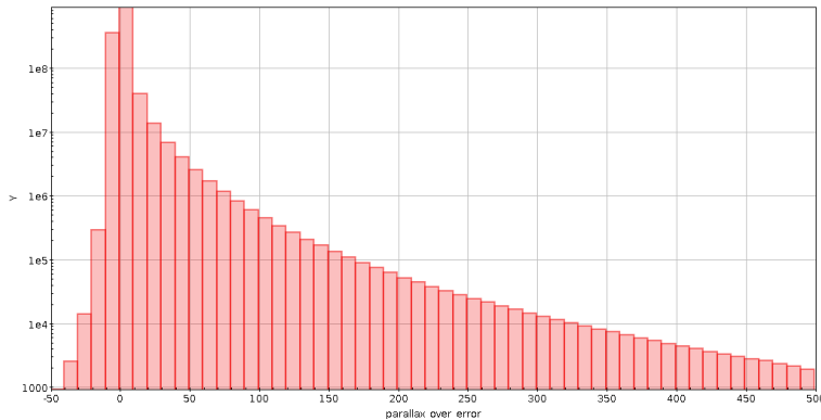
Figure 3: Distribution of the relative accuracy of the parallaxes in the Gaia survey, given as \varpi/\sigma_\varpi . There are about 50 millions stars with a parallax with a relative accuracy better than 10%. Credit: ESA/Gaia/DPAC
