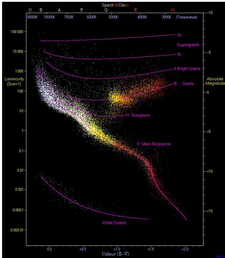
Figure 4: An observational Hertzsprung–Russell diagram with 22,000 stars plotted from the Hipparcos Catalogue and 1,000 stars from the Gliese Catalogue of nearby stars.
