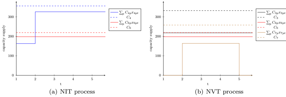
Figure 5: Capacity-allocation decisions from multi-period modeling approach versus the apriori capacity C_l for 5-4/8/20-25-(I1,LT,TC,.)
