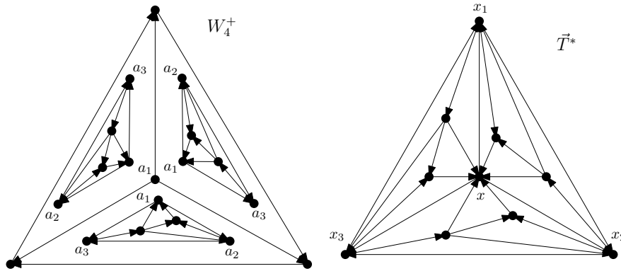
Fig. 2: Left: Gluing three copies of \vec{T} into the faces of W_4^+ . Right: The arising directed planar triangulation \vec{T}^* .
