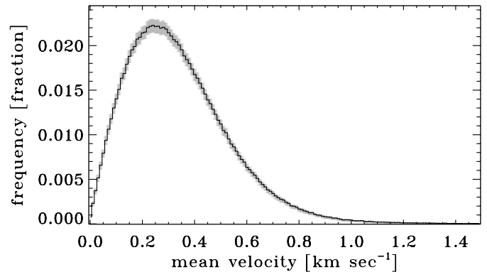
Fig. 4. Histogram of all measured mean horizontal velocities (both in x and y direction), with 3\sigma estimates (shaded contours). Most velocities are below 1 \text{ km s}^{-1} , with a maximum around 0.25 \text{ km s}^{-1} .
