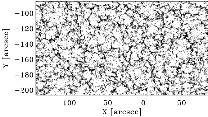
Fig. 5. This plot shows the final positions of about 30 000 “corks” or tracers after 4 hours, that were initially distributed regularly and allow to freely flow on the velocity fields. Some tracers have not yet reached their final destination, but large scale structures are visible. Axes: X and Y in arcsec from disk center.
