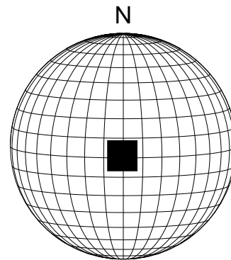
Fig. 1. Solar location of the field observed with TRACE on October 14, 1998, slightly off disk center. Only the lower half of this field was used for the analysis presented in this paper. The grid shows heliocentric longitude and latitude.
