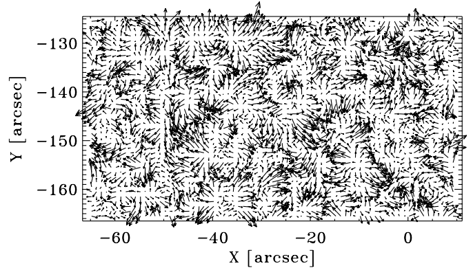
Fig. 3. Horizontal flows in a partial cutout from the measured horizontal velocity field at 1 arcsec resolution between 10:10–10:15 October 14 1998. Each arrow shows the direction and magnitude of the velocity at a particular point with 1 arcsec length corresponding to 0.25 \text{ km s}^{-1} . Axes: X and Y in arcsec from disk center.
