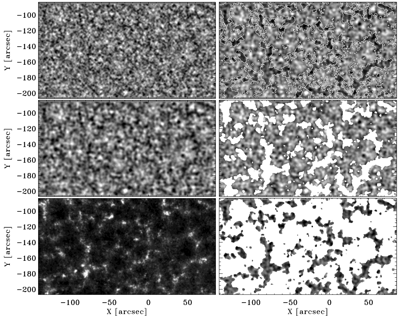
Fig. 6. Top left: classic divergence defined by Eq. (1) averaged over the entire duration (228 min) of the observation. Bright areas indicate locations where the flows are diverging, dark areas indicate converging flows. Middle left: same as first panel, but showing isotropic divergence as defined by Eq. (2). Large scale structures become more distinct. Bottom left: the average of the 1700 Å sequence taken at the same time and location. The greyscale is logarithmic in order to bridge the large contrast. Top right: again showing the time-averaged isotropic divergence but now overlaid with the contours of the bright network from the bottom-left panel. A clear correlation between the dark converging areas and the bright network can be seen. Middle and bottom right: split of the top-right panel into internetwork-only and network-only displays, using a mask defined by the network contours. The split produces yet clearer visualisation of the spatial correlation between the dark converging areas and the bright network. Axes: X and Y in arcsec from disk center, all panels show the same subfield.
