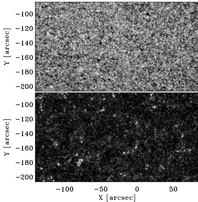
Fig. 2. Top: sample white-light image taken by TRACE at 10:03 UT, Oct. 14 1998. With a resolution of only 1 arcsec TRACE only resolves the larger granules. Smaller granules can jointly appear erroneously as large granules when close enough. No large-scale or magnetic structures are discernable. Bottom: corresponding 1700 Å image taken by TRACE 2 s earlier. The brightest features belong to the chromospheric network. The latter stands out more clearly in the time-average display at bottom-left in Fig. 6. Axes: X and Y in arcsec from disk center.
