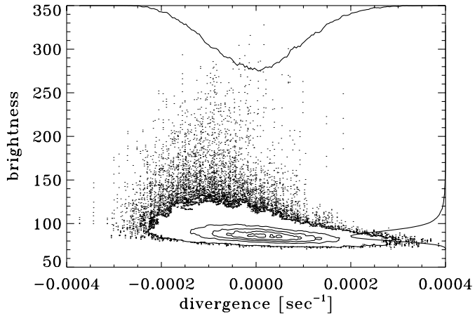
Fig. 7. Correlation between average 1700 Å brightness and average velocity field divergence shown as a pixel-by-pixel scatter plot, with density contours replacing individual points where they become too close. The curves along the axes measure the first moments per row and column, respectively. The locations with the brightest network (upward tail of the scatter cloud) correspond to negative divergence in the flow field.
