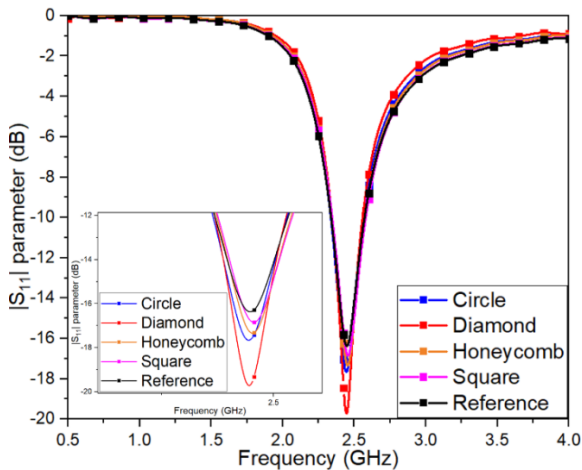
Fig. 5: Reflection parameter |S_{11}| for meshed antenna with a pitch p of 0.95 mm and a total width w of 1.15 mm. In the insert, zoom of the coefficient at 2.45GHz.
