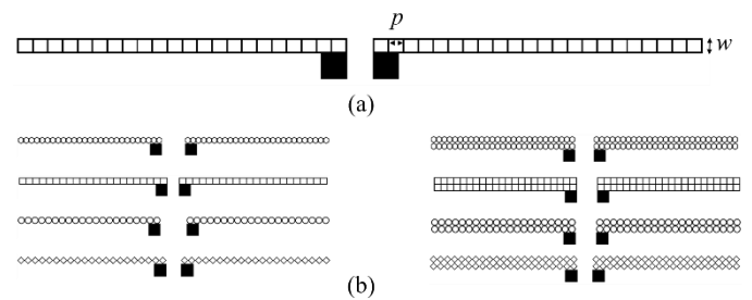
Fig. 1: (a) Geometry of a mesh square dipole antenna with a pitch p and a width w . (b) Design of dipole antenna with different width w and mesh geometry: honeycomb, square, circle and diamond. On the left, the first type for w/2 . On the right, the second type for w .
