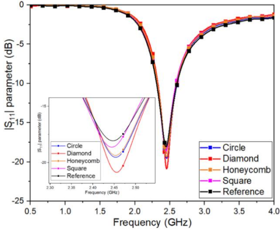
Fig. 4 : Reflection parameter |S_{11}| for meshed antenna with a pitch p of 1.9 mm and a total width w of 2.3 mm. In the insert, zoom of the coefficient at 2.45GHz.
