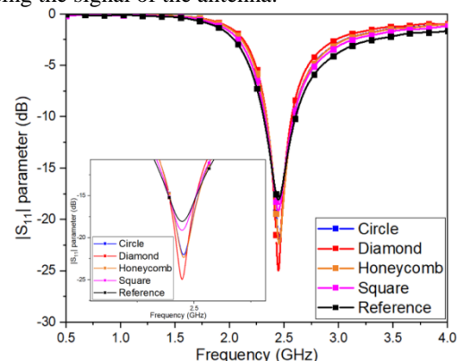
Fig. 3: Reflection parameter |S_{11}| for meshed antenna with a pitch p of 2.1 mm and a total width w of 2.3 mm. In the insert, zoom of the coefficient at 2.45GHz.
